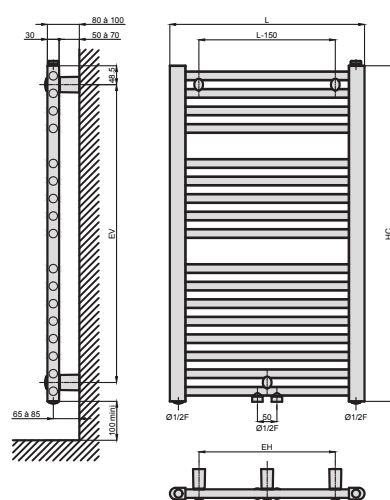
VERSION EAU CHAUDE RACCORDEMENT CENTRAL 50 MM
