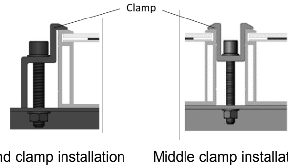
Figure 2. PV module installed with clamp fitting method
