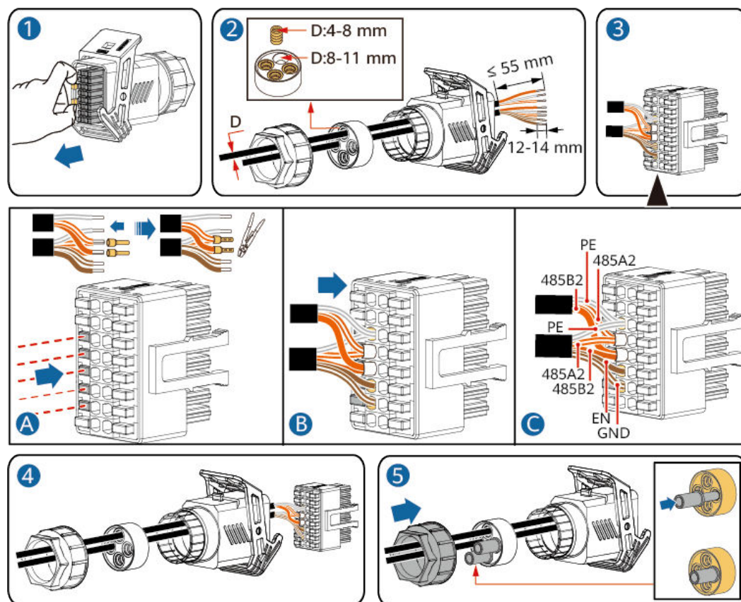
Figure 5-28 Installation des câbles
