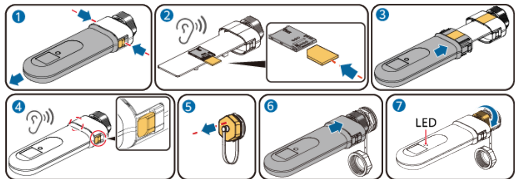
Figure 5-47 Installation du Smart Dongle 4G (SDongleB-06)
