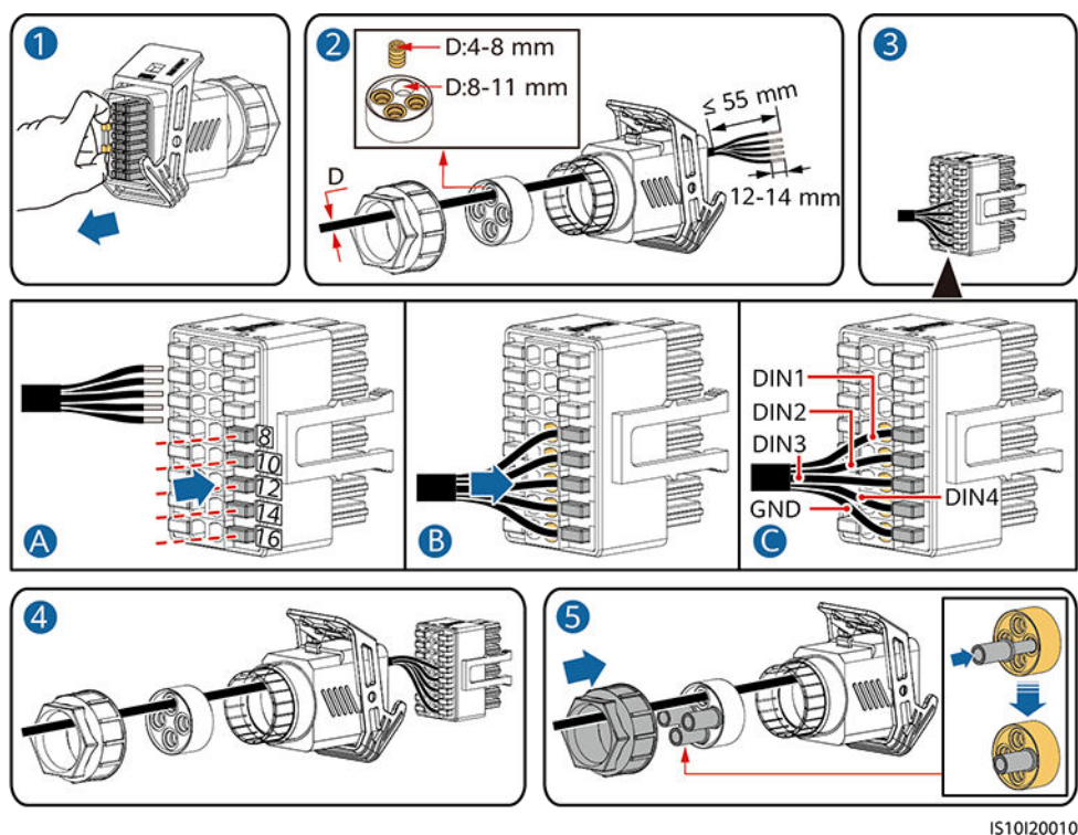
Figure 5-40 Installation du câble
