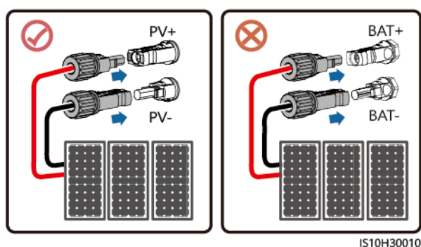
Figure 5-12 Connexion
