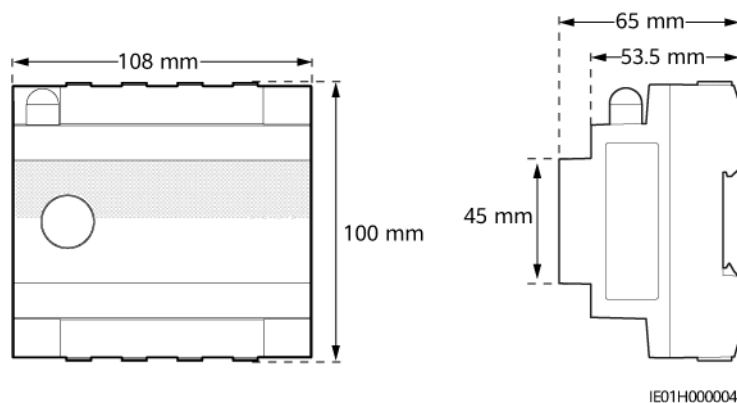
Figure 4-1 Conditions d'installation
